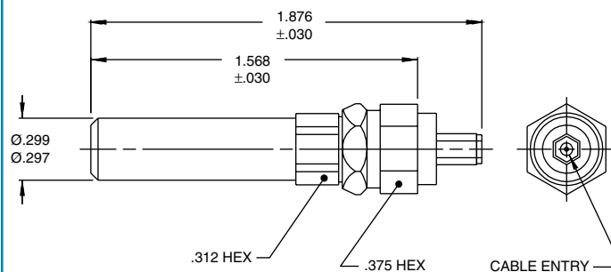
Patch Plug Mini-WECO BNC Strip dimension Crimp Contact, Crimp Shield
