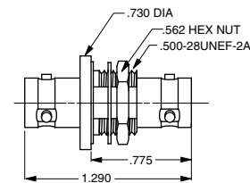
BJ78HS BJ378HS (Threaded Version Not Shown)
