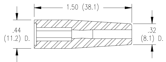
Dimensions 1-8065-10 (for cable groups 734, 735, Belden 1694A, Belden 1855A)
