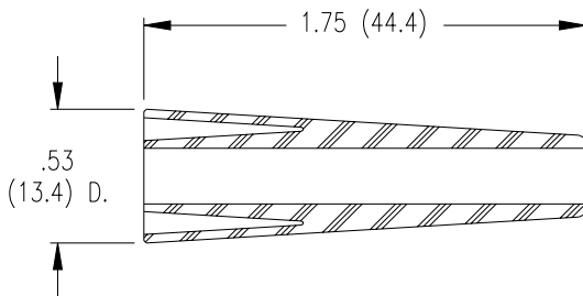
Dimensions 1-1483-10 (for cable groups RG-58/U, RG-59/U, RG-174/U)
